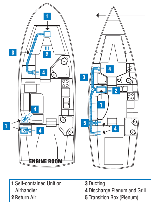
Figure 3: Comparison of typical remote and self-contained systems
