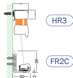
3 BAR FACE FIXED BLIND Types: AO-DB, AO-DBE, AB, DB, DBE, PB
