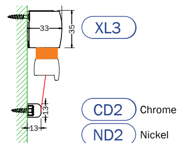
2 BAR DOME FACE FIXED BLIND Types: A0-DB, A0-DBE
