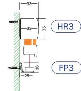
2 BAR FOOTPLATE FACE FIXED BLIND Types: A0-DB, A0-DBE
