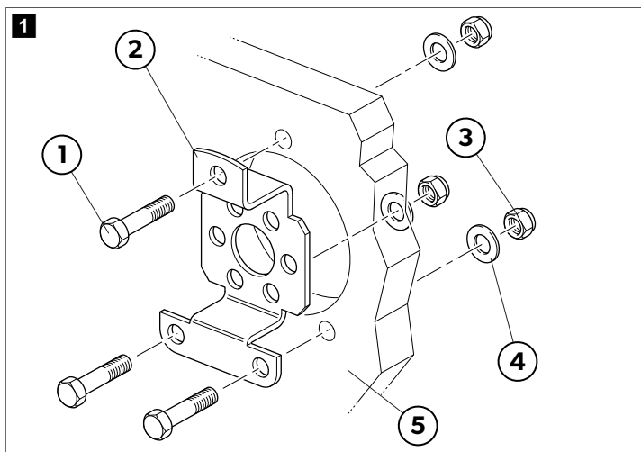
90° kronstein
