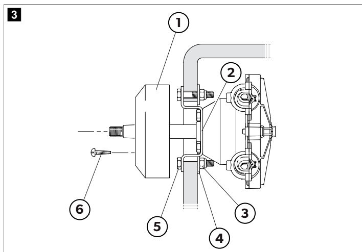
SH5150-roret vises
